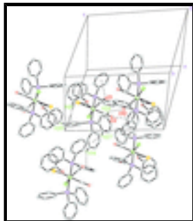
Fig. 3. The packing diagram of (I), showing the intermolecular C—H \cdots O, C—H \cdots \pi (arene) hydrogen bonds and CO \cdots \pi (arene) interactions.
